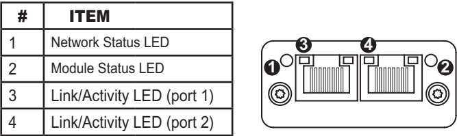
Fig. 10-6 – Front panel connectors and LEDs
